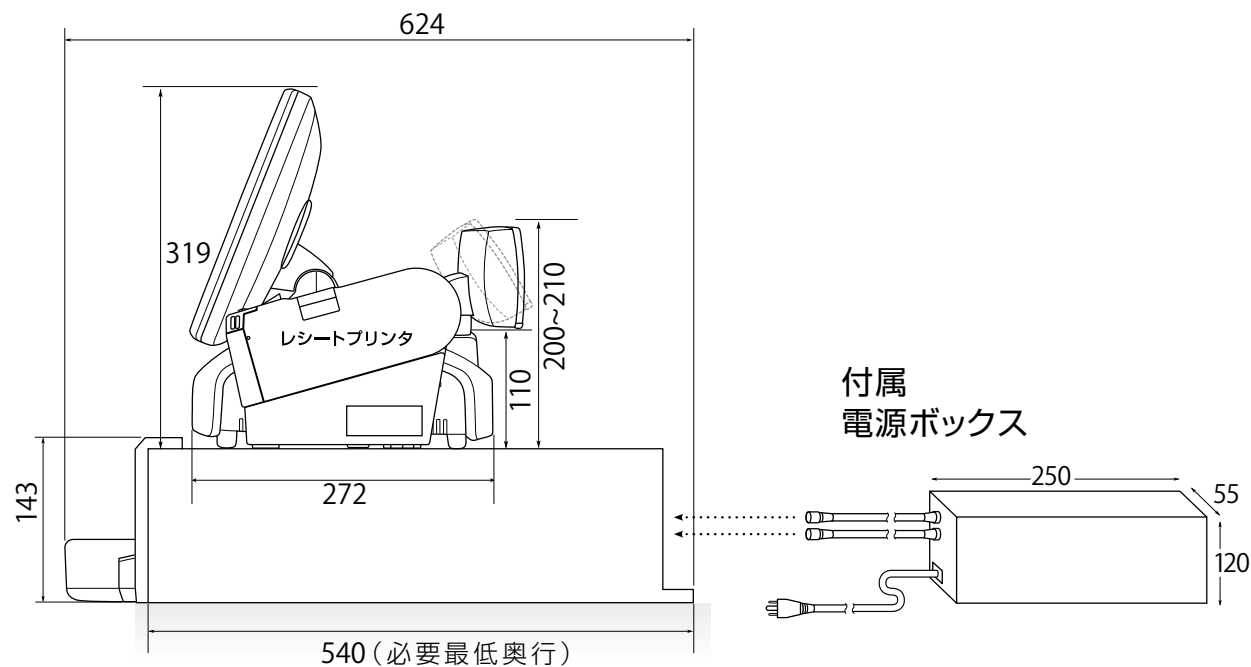
SIDE VIEW
